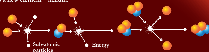
Nuclear Fusion
